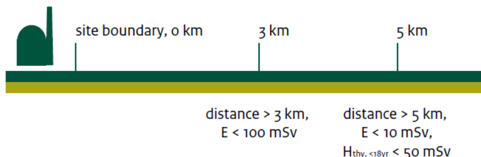
Figure D.1. Zones and intervention levels for postulated core-melt accidents.
