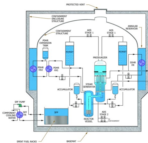
Figuur III.8 Holtec LWR SMR concept
